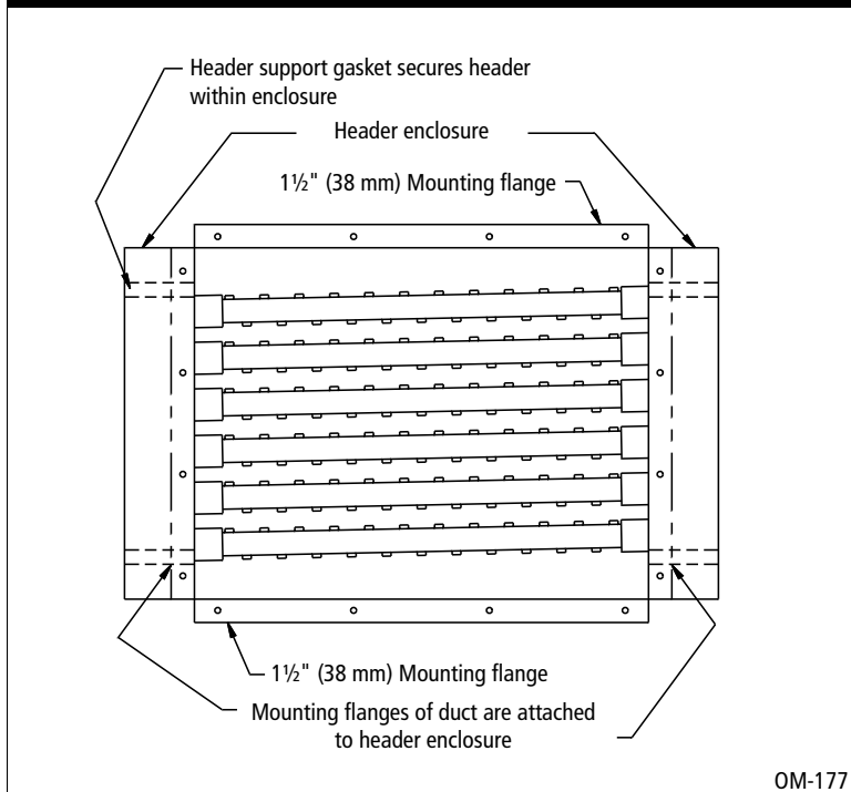
Figure 13-1: Elevation view - Model LH
