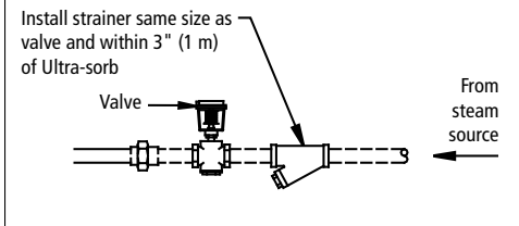
Figure 17-1: Ultra-sorb strainer
