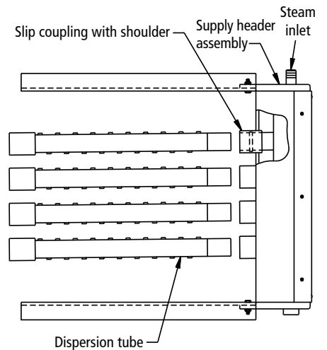
Figure 5-3: Dispersion tubes
