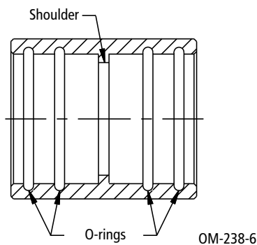
Figure 8-3: Detail view of slip coupling
