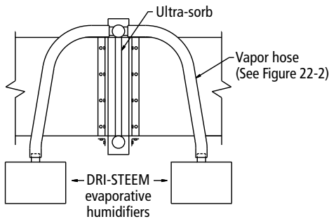
Figure 18-1: Vapor hose
