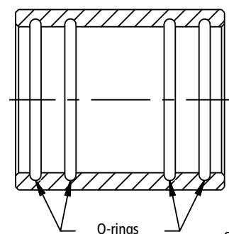
Figure 5-5: Slip coupling without shoulder
