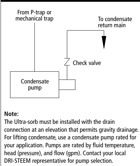
Figure 16-4: Lifting condensate
