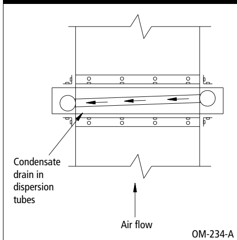
Figure 14-1: Elevation view - Model VAF (for vertical airflow)
