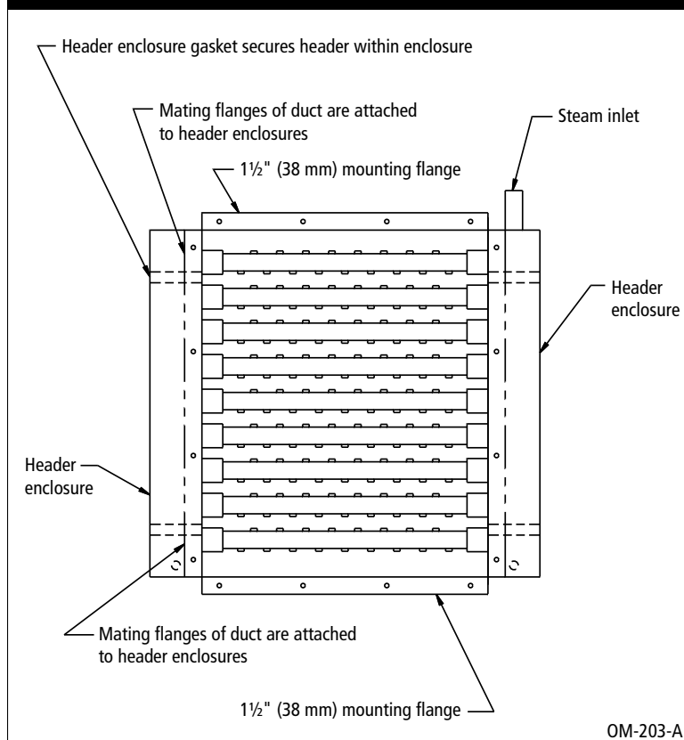
Figure 14-3: Plan view - Model VAF
