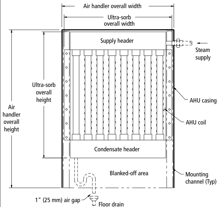
Figure 15-1: Ultra-sorb installed inside an air handler
