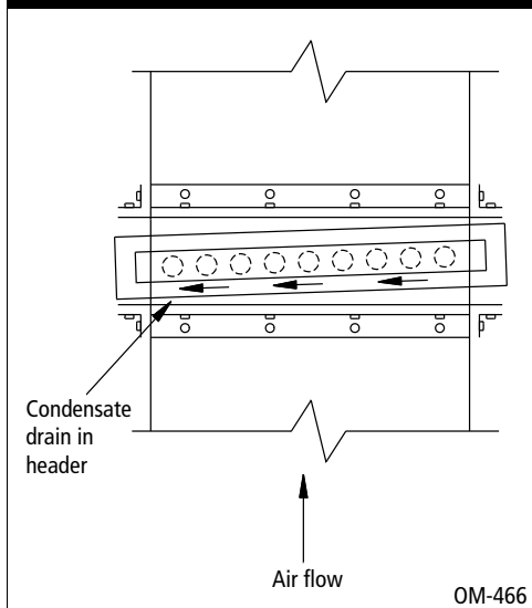
Figure 14-2: Side view - Model VAF
