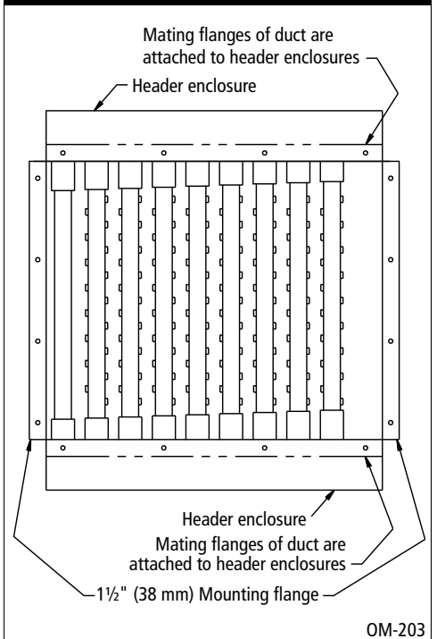
Figure 13-3: Plan view - Model LH
