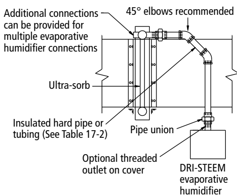
Figure 18-3: Threaded connections
