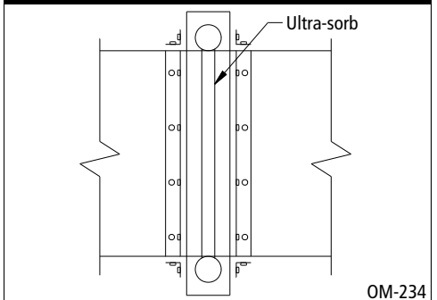
Figure 13-2: Elevation
