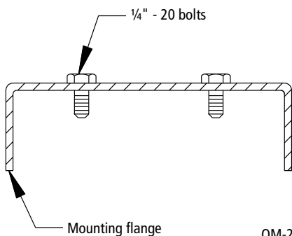
Figure 8-2: Detail view of mounting flange
