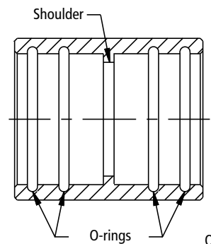
Figure 5-4: Slip coupling with shoulder
