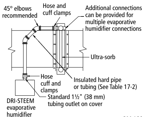
Figure 18-2: Hose cuff installation
