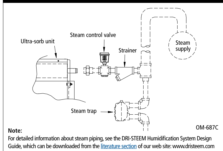
Figure 16-1: Connection to a boiler (pressurized steam applications)
