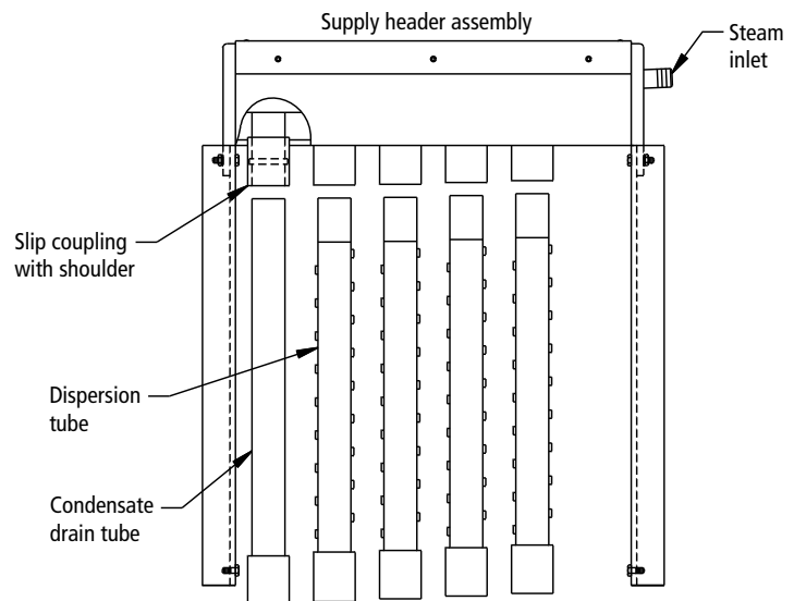
Figure 8-4: Dispersion tubes
