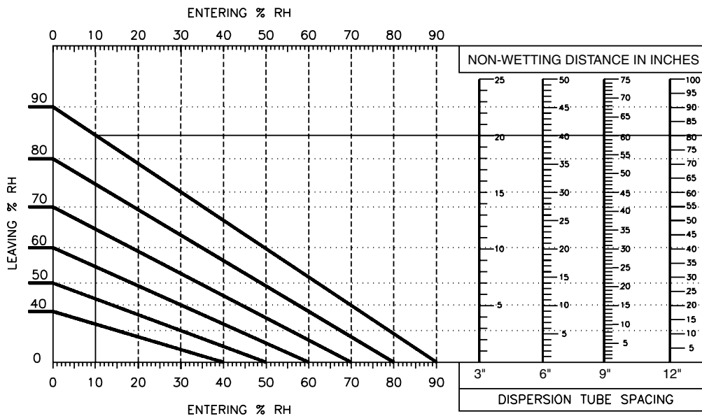
Figure 22-1: Ultra-sorb non-wetting distances
