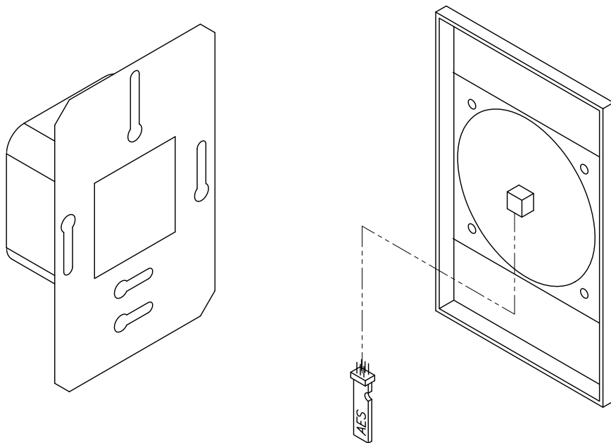
FIGURE 22-1: ACCESSING THE INTERNAL HUMIDITY SENSOR
