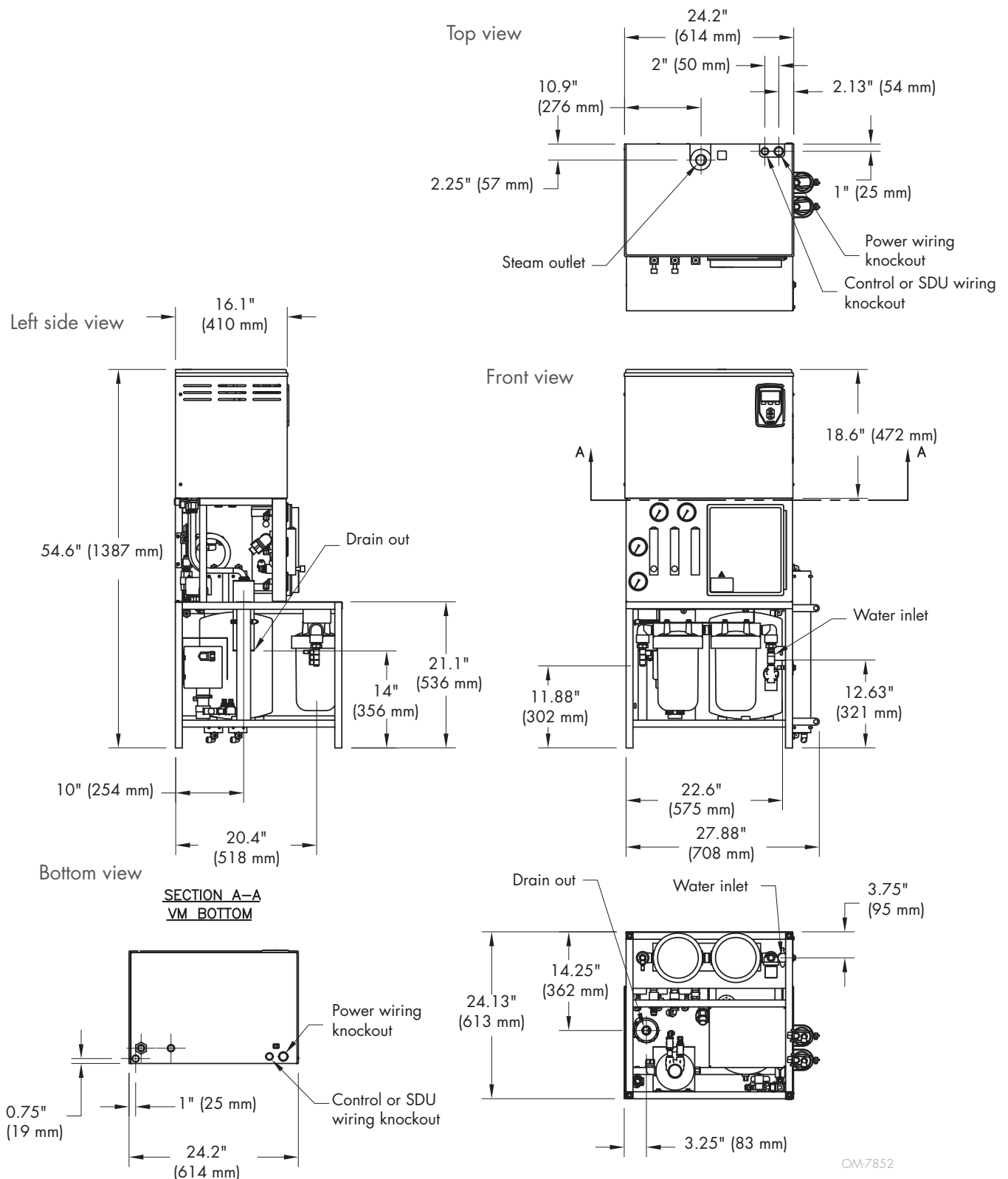
Figure 1-1: Low maintenance humidifier dimensions
