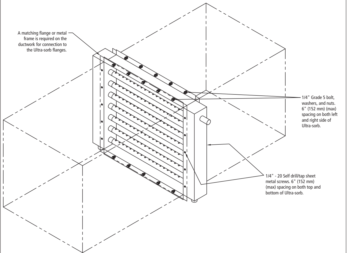
Figure 1-1: Ultra-sorb model LH installation in a duct
