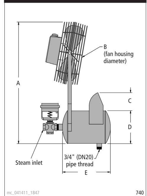
Figure 1-2: Area-type humidifier dimensions
