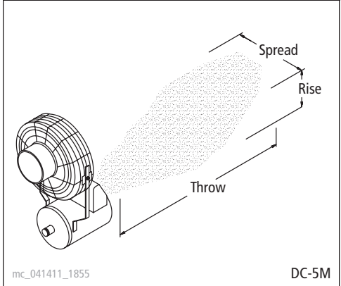
Figure 2-1: Area-type rise, spread, and throw
