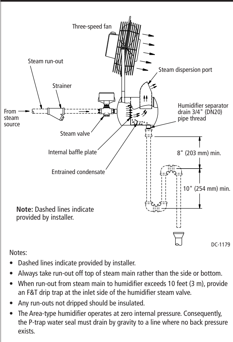
Figure 1-1: Area-type humidifier
