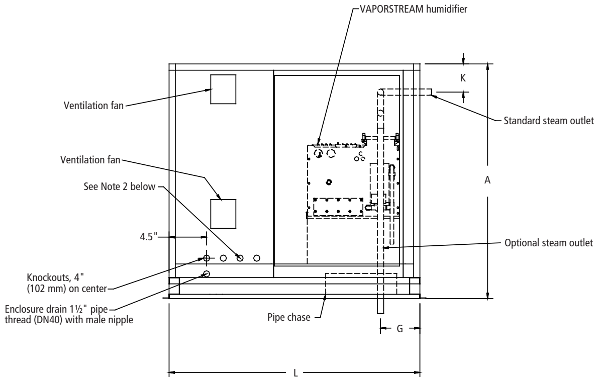
Figure 7-1: VAPORSTREAM outdoor enclosure with standard or optional steam outlet, elevation view
