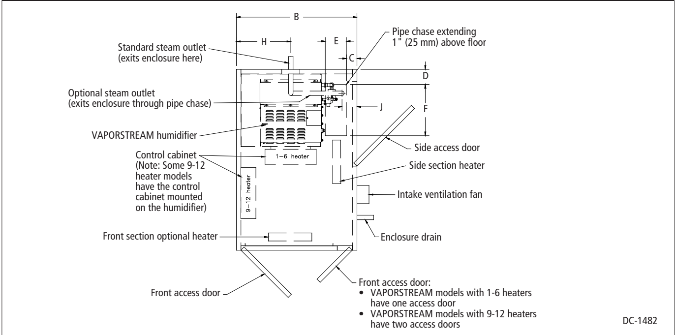
Figure 8-1: VAPORSTREAM outdoor enclosure, top view
