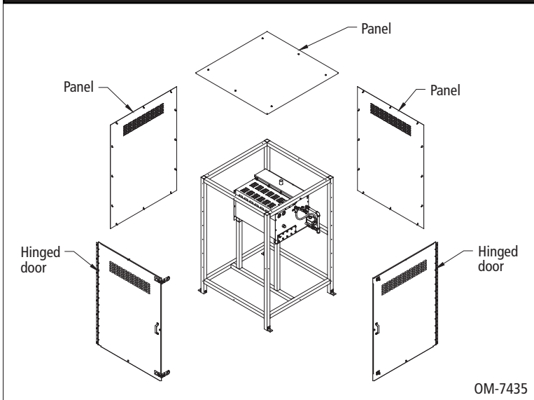
Figure 5-1: Weather cover exploded view
