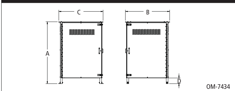
Figure 5-2: Weather cover dimensions
