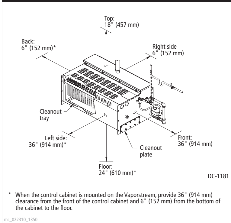
Figure 4-1: Vaporstream clearance recommendations
